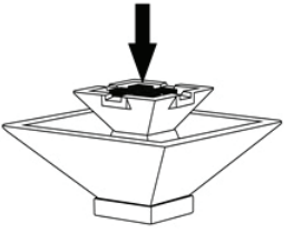
FT-348A (3 lbs) 5.25"L x 5.25"W x 1.5"H
