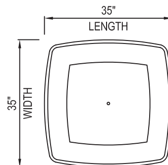
PLAN VIEWS
