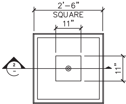
1 PLAN VIEW SCALE: 1/2"=1'
