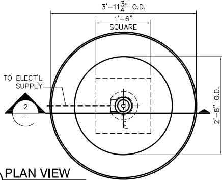
1 PLAN VIEW
