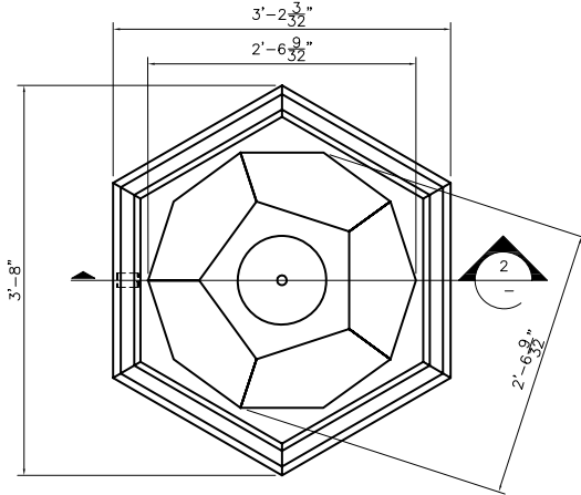
1 PLAN VIEW
