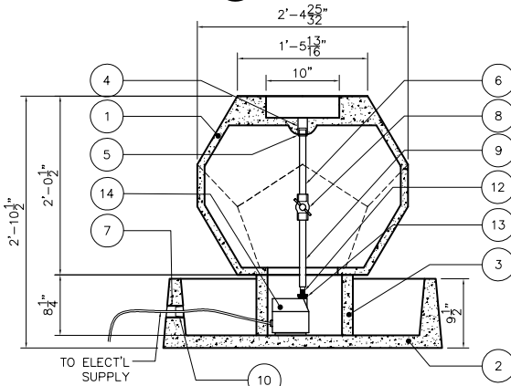
2 SECTION
